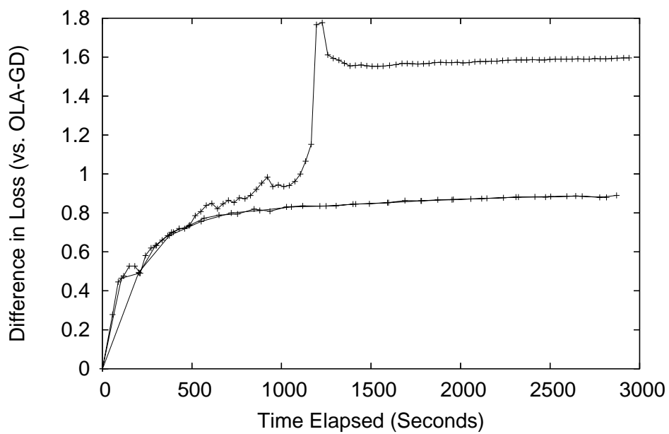
Distributed SGD: SVM
