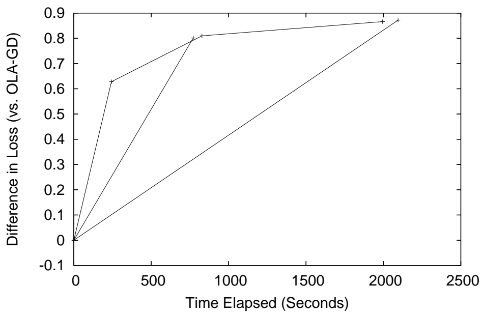
Distributed Mini-Batch: SVM
