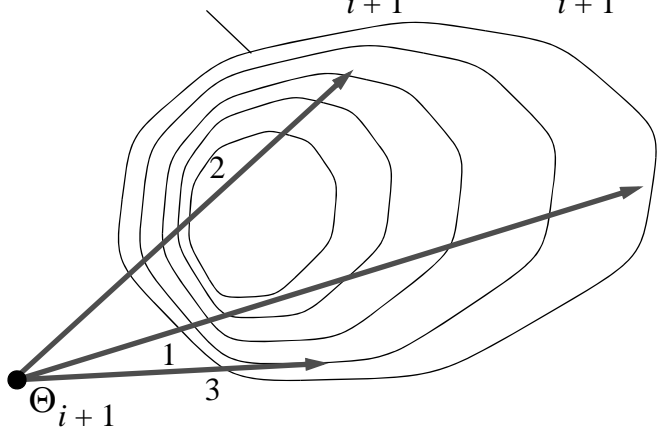
(b) Three sampled values for \Delta_{i+1}
