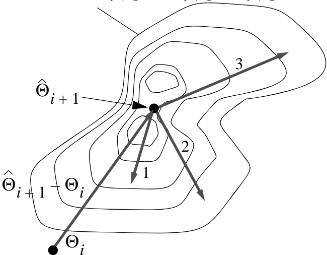
(a) Three sampled values for \varepsilon_{i+1}
