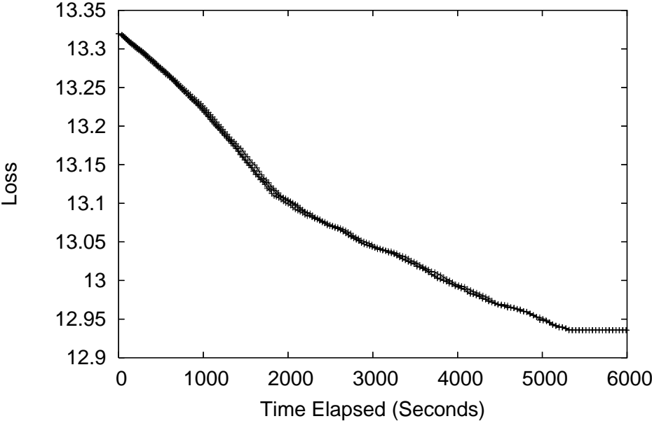
OLA-GD: Linear Regression
